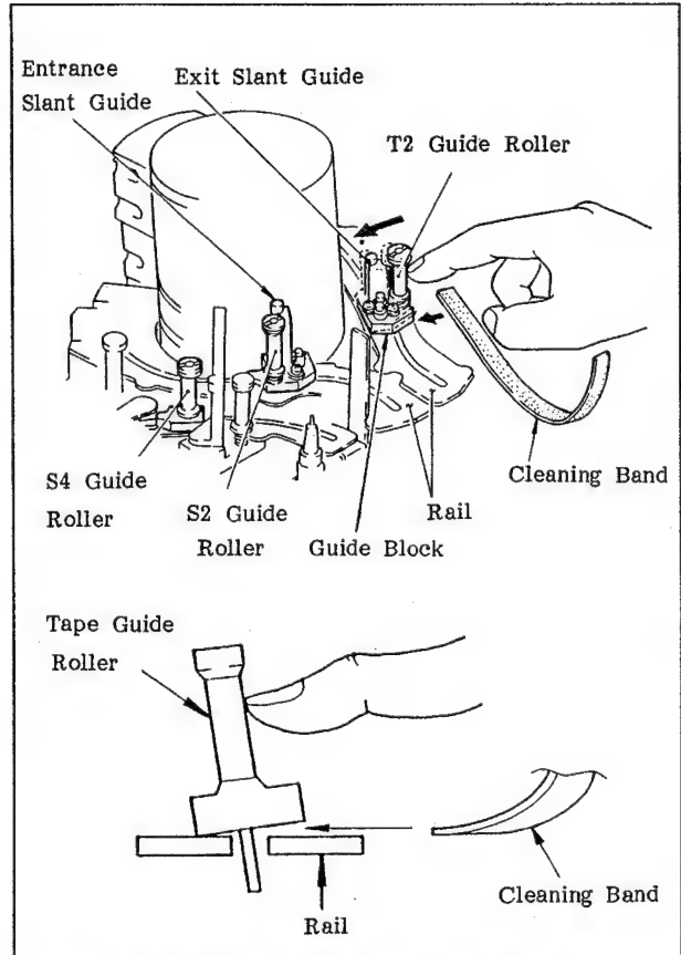
Fig. 5-10 Cleaning the Slider Guide Blocks (1)
